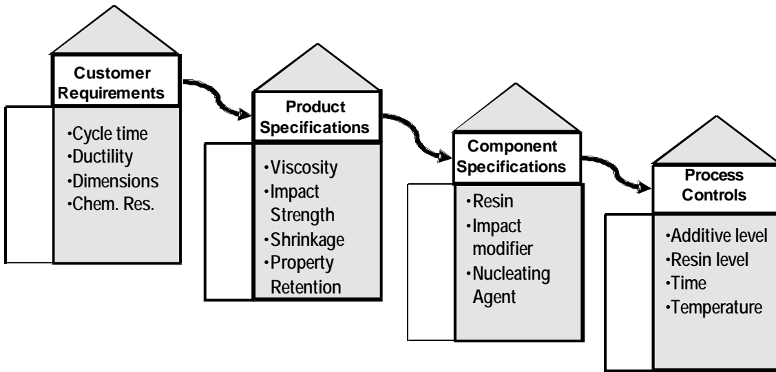
Figure 3 – Critical Parameter Drilldown form Customer Requirements using a QFD
